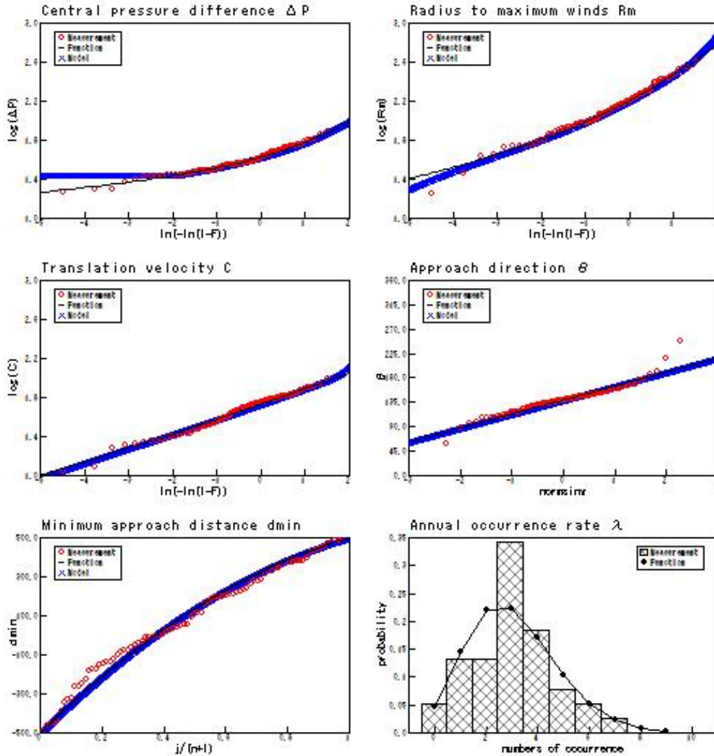
Comparison between the measured probability distribution of tropical cyclone parameters and the model function
