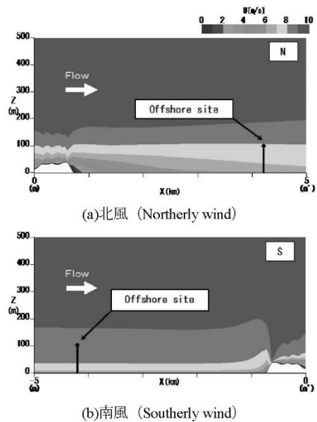
図 2 洋上風力発電所地点における風速の空間分布 (Spatial distributions of wind speed at the offshore site for the northerly and southerly winds)
