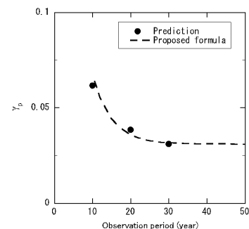
図 17 年最大風速の 50 年再現期待値の変動係数と気圧の観測年数との関係 (Relationship between a coefficient of variation of 50-year recurrence wind speed and observation period of pressure)
