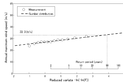
図 5 温帯低気圧の年最大風速の予測値と観測値との比較 (Comparison of predicted and observed extreme wind speeds caused by extratropical cyclones)
