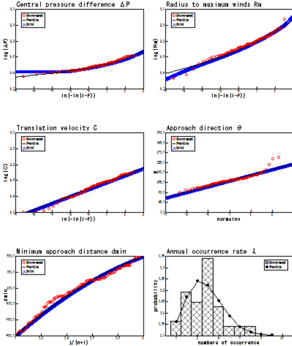
Comparison between the measured probability distribution of tropical cyclone parameters and the model function
