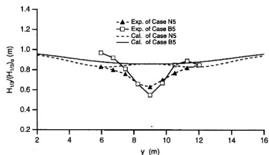
Fig.15 Comparirion of normalized wave heights along transect 4
